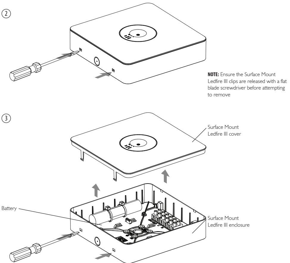
Figure 1 : Surface Mount Ledfire III disassembly and installation
